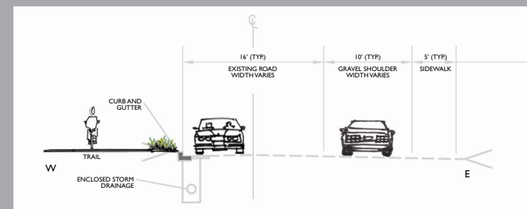
Lincoln Ave Improvements - Typical Section
