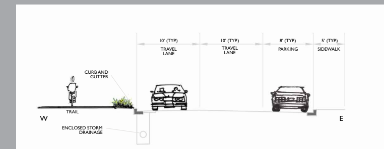
Lincoln Ave Improvements - Future Section
